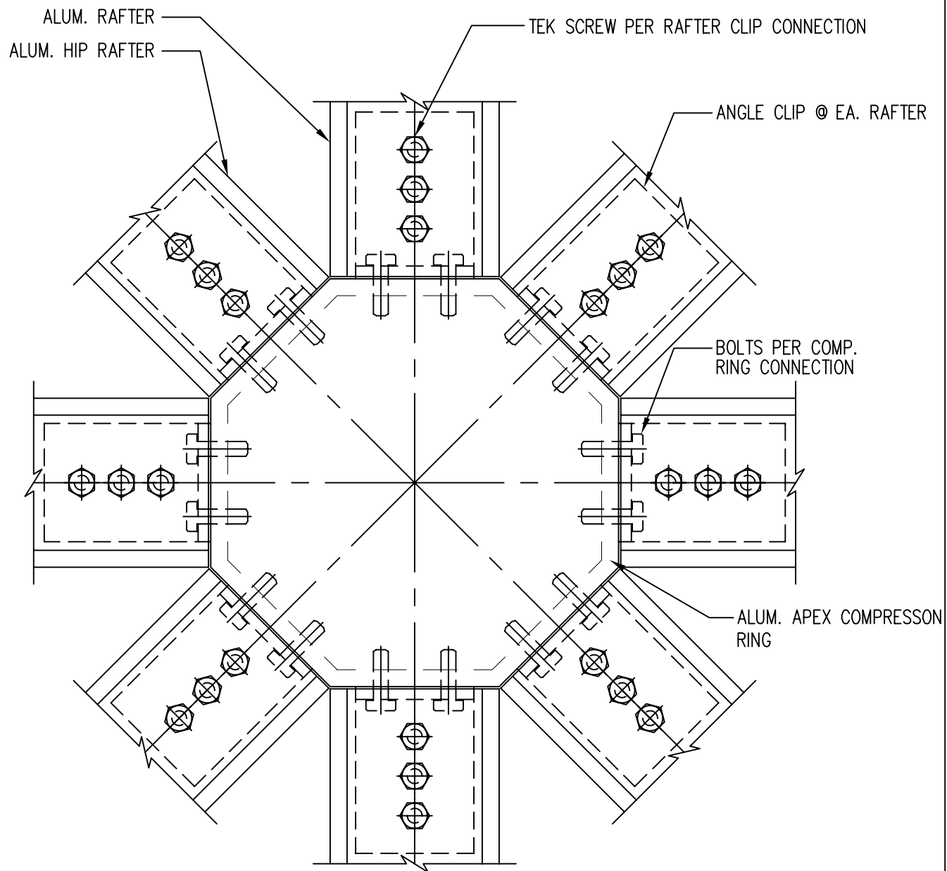
APEX PLAN HALF SCALE
