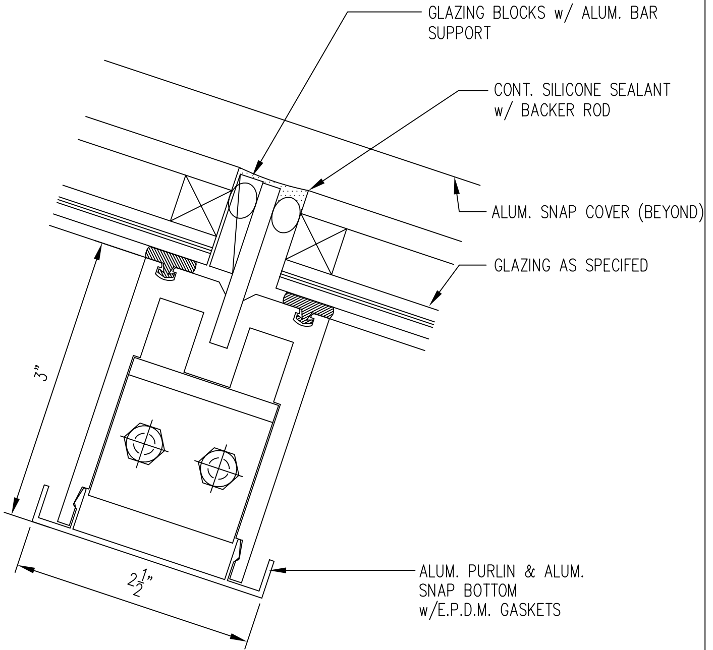
3" PURLIN B1 FULL SCALE:
