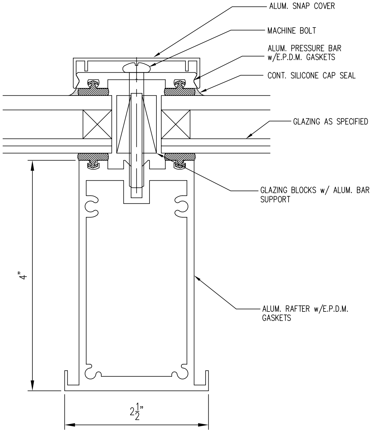
4" RAFTER A FULL SCALE:
